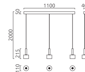
3 x E14 mattnickel / nickel mat 36/2104.06/5306 mattschwarz / black mat 36/2104.22/5306
