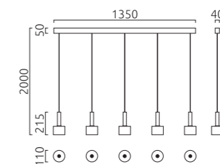
5 x E14 mattnickel / nickel mat 56/2104.06/5306 mattschwarz / black mat 56/2104.22/5306
