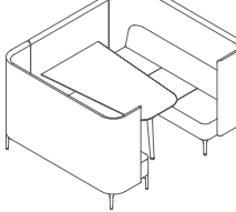
PULBW3H Pullman 3 Seat Booth Wide mm W 2250 D 1900 H 1300 Seat 450 inch W 88.5 D 75 H 51 Seat 18
