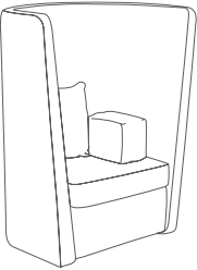
NOBSN11 Busby Chair Left Hand with Cushions mm W 850 D 650 H 1300 Seat 430 inch W 33.5 D 25.5 H 51 Seat 17
