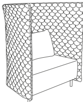
CLOQ15H Cloud Quilt 1.5 Seat Sofa with High Back mm W1100 D750 H1300 Seat 400 inchW43.5 D29.5 H51 Seat15.5
