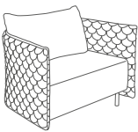
CLOQ15L Cloud Quilt 1.5 Seat Sofa with Low Back mm W1100 D750 H650 Seat 400 inchW43.5 D29.5 H25.5 Seat15.5
