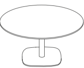
MP105D Megaped 1050 Circular Table mm Dia 1050 H 750 inch Dia 41.5 H 29.5
