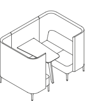
PULB2H Pullman 2 Seat Booth mm W 1950 D 1300 H 1300 Seat 450 inch W 77 D 47 H 51 Seat 18
