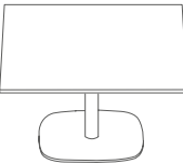
MP115S Megaped 1150 Square Table mm W 1150 D 1150 H 750 inch W 45.5 D 45.5 H 29.5
